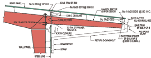
DETAIL 'A' OVERHANG CANOPY AT RY-FRAME SIDEWALL
