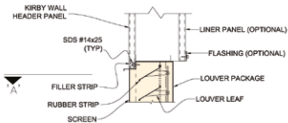
HEAD SECTION -NORMAL
