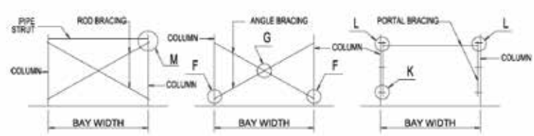
BRACINGS AT SIDEWALL
