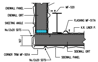
DETAIL "A3" BY-FRAME MAIN END CORNER COLUMN
