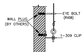
OPERATOR CORD ATTACHMENT TO MASONRY WALL
