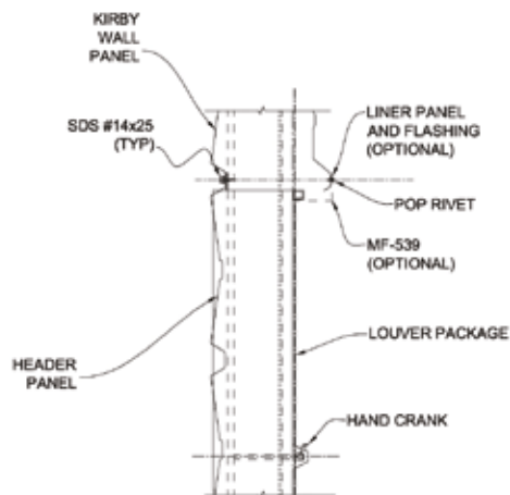
SECTION - 'A'
