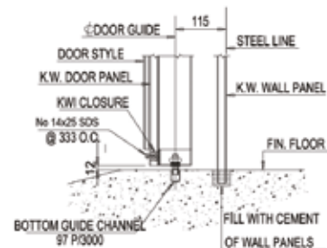
SECTION - N
