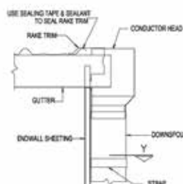
SECTION X
