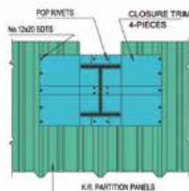
SECTION - 6
