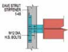
SECTION - 1
