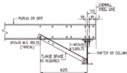
PURLIN CONNECTION DETAIL At Lines 1 & 9
