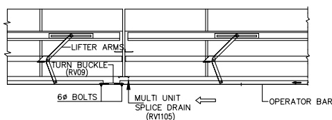
OPERATOR BAR CONN. AT MULTI UNITS
