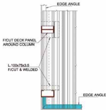
DETAIL - F PLAN AT WIND COLUMNS
