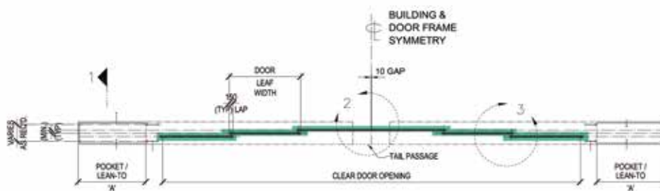
DOOR LEAF PLAN
