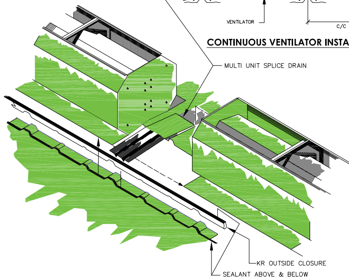
CONTINUOUS VENTILATOR INSTALLATION
