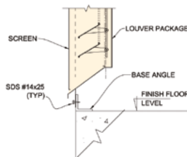
SILL SECTION -FLOOR POSITION
