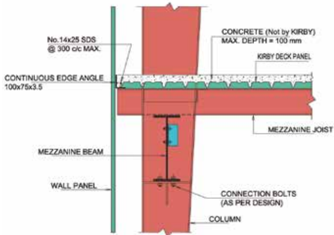
DETAIL - D MEZZANINE BEAM FRAMING TO COLUMN WEB
