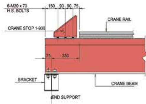
DETAIL AT CRANE STOP
