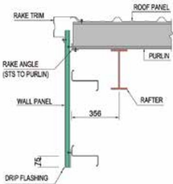
SECTION - "X"
