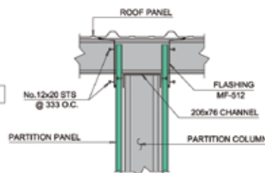
SECTION - 3
