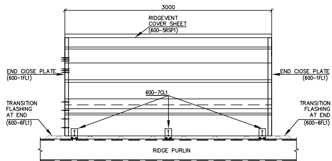
SIDE VIEW (SINGLE UNIT)
