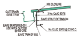
DETAIL 'K' SECTION THRU' EAVE OF PURLIN EXTENSION WITHOUT SOFFIT
