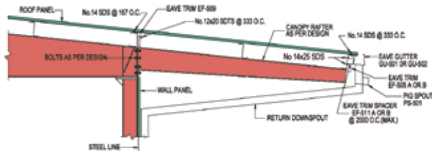
DETAIL 'B' OVERHANG CANOPY AT RY-FRAME SIDEWALL (ALL OTHER DETAILS SAME AS IN DETAIL 'A')
