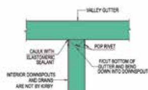
DOWNSPOUT INSTALLATION
