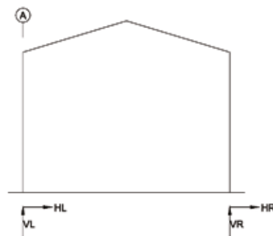
MAX WIND COL REACTIONS (KNS)
