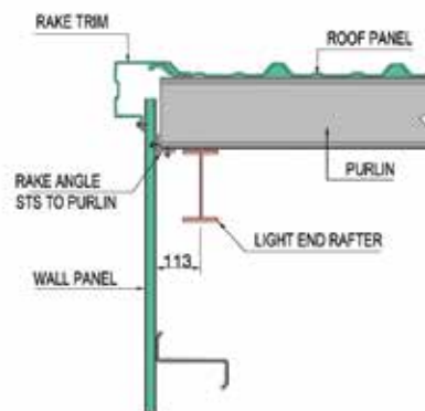
SECTION 'X'
