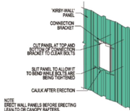
DETAIL 'B' CUTTING DETAILS FOR K.W. PANELS
