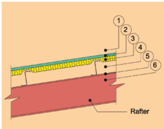
AT ROOF
