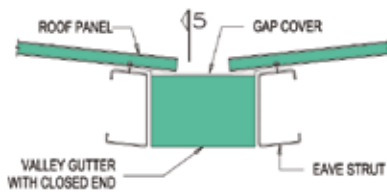
DETAIL 'F' AT VALLEY GUTTER
