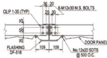
SECTION - H
