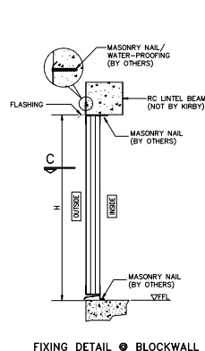
FIXING DETAIL @ BLOCKWALL
