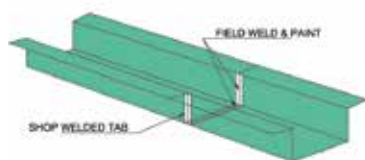
FIELD SPICE FOR 1.0 mm Thk. OR HEAVIER GUTTERS
