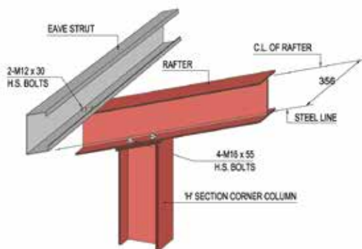
DETAIL 'A' EAVE STRUT & RAFTER CONNECTION TO 1/2 SECTION CORNER COLUMN
