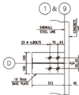
DETAIL 'D'
