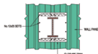
SECTION '2'
