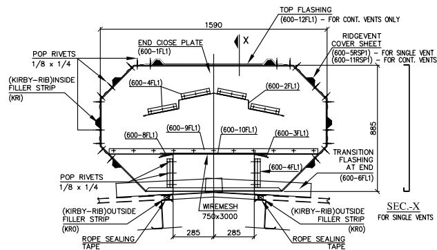
RIDGE VENT. ASSEMBLY
