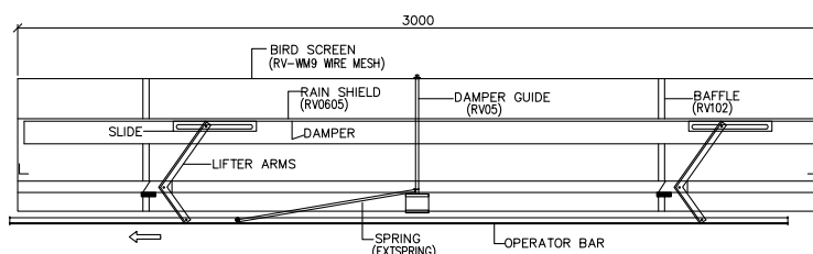
SECTIONAL ELEVATION
