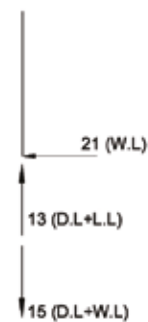
MAX WIND COL REACTIONS (KNS)
