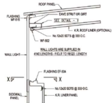
DETAIL 'F' SECTION AT SIDEWALL WITH WALL LIGHT
