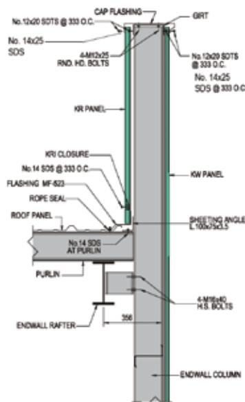
DETAIL 'B' SECTION AT ENDWALL
