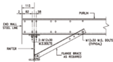
PURLIN CONNECTION DETAIL AT GRID LINE 1 & 9
