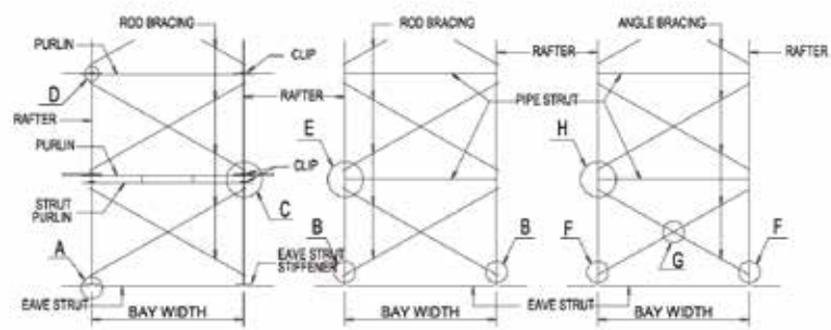
BRACINGS AT ROOF
