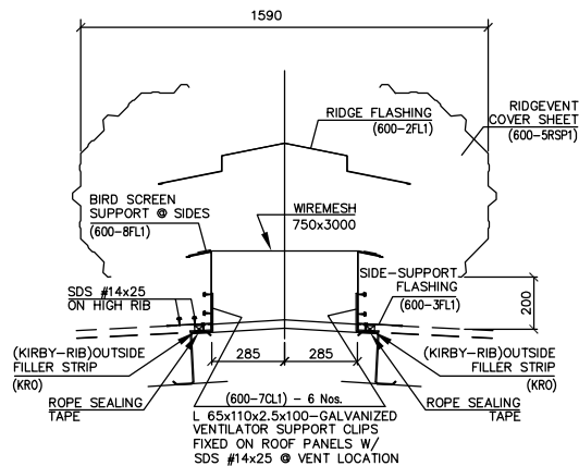
RIDGE VENT. FIXING DETAIL
