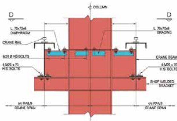
DETAIL 'C'
