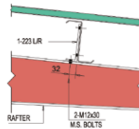
SECTION 1
