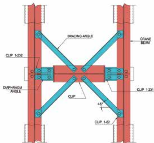
PLAN B-B
