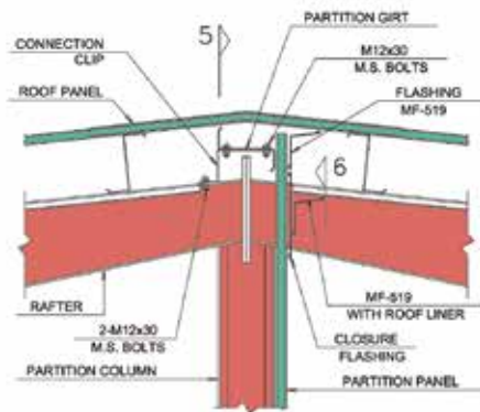
DETAIL 'E' TRANSVERSE SECTION SHOWING PARTITION SUPPORT & SHEETING AT PEAK
