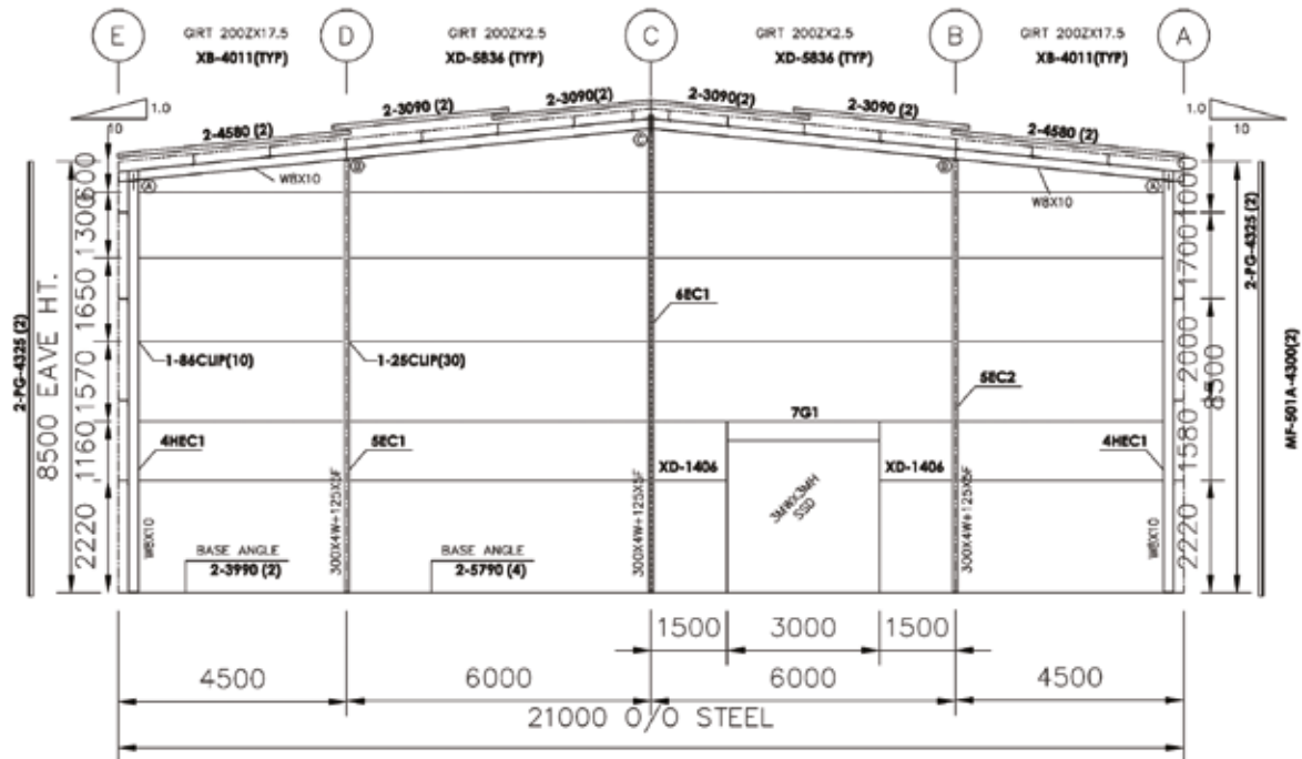
END WALL FRAMING ELEVATION @ GRID 1
