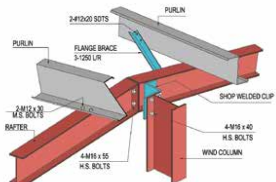
DETAIL 'C' PURLINS & RAFTER CONNECTION TO 1/2 SECTION COLUMN ON PEAK LINE
