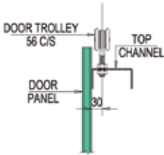
SECTION - D
