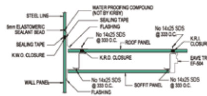
DETAIL 'E' PANEL & TRIM INSTALLATION
