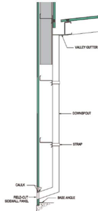
DETAIL 'C' DOWNSPOUT INSTALLATION
