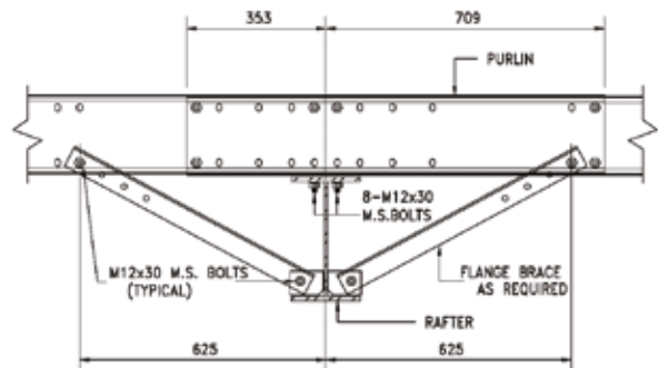
PURLIN CONNECTION DETAIL At Lines 2 & 8
