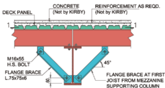
DETAIL - A AT INTERMEDIATE BEAM
