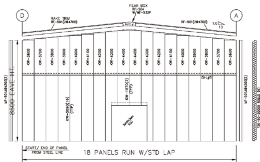
END WALL SHEETING ELEVATION @ GRID 1
