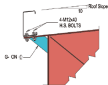
DETAIL AT EAVE
