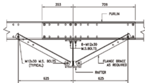
PURLIN CONNECTION DETAIL At Lines 2 & 6
