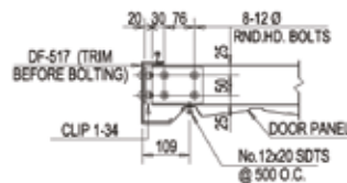
SECTION - F
