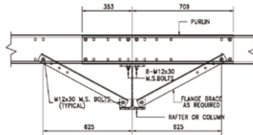
PURLIN CONNECTION DETAIL At Lines 2 & 6
