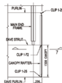
DETAIL 'D'
