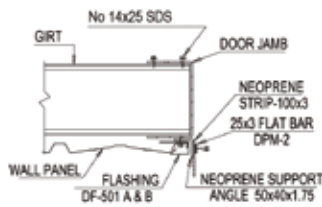
SECTION - L
