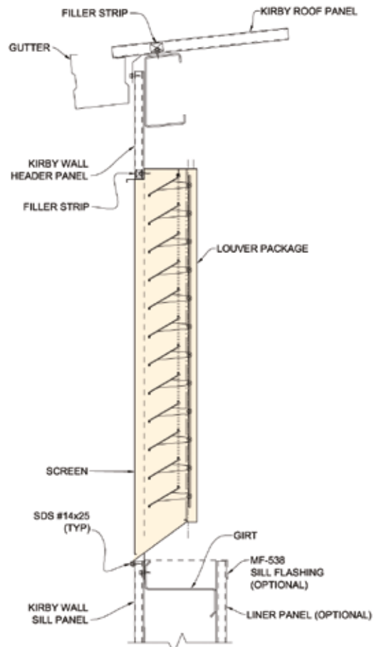
HEAD SECTION -AT EAVE STRUT
