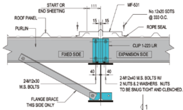
DETAIL 'A' AT PURLIN & ROOF PANEL
