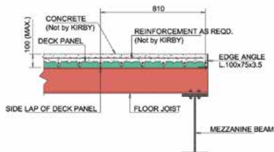
DETAIL - J PANEL SIDE LAPS
