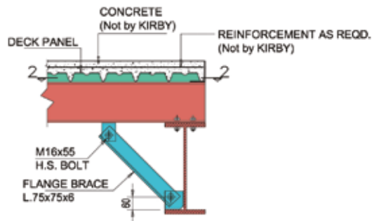
DETAIL - B AT END BEAM
