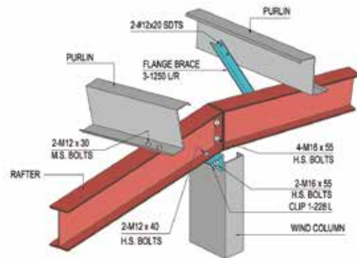
DETAIL 'G' PURLINS & RAFTER CONNECTION TO 'C' COLUMN ON PEAK LINE
