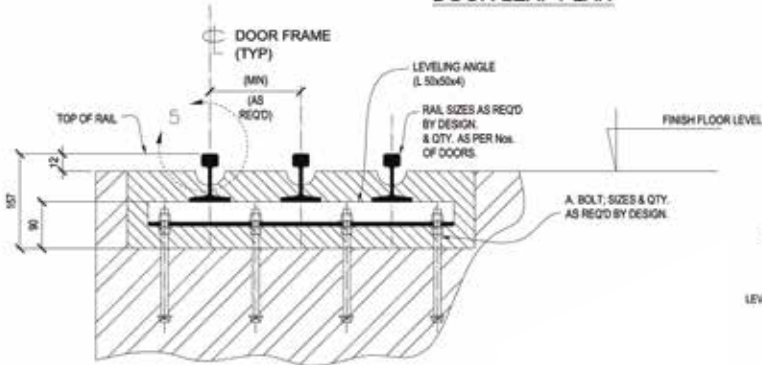
SECTION: 1
