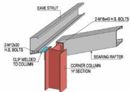
DETAIL 'A1' EAVE STRUT & BEARING RAFTER CONNECTION TO 14' CORNER COLUMN
