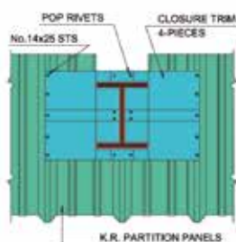
SECTION - 6
