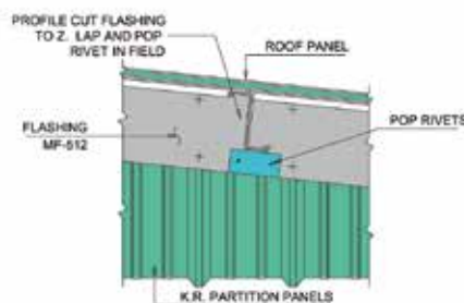
SECTION - 3
