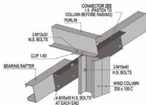
DETAIL 'B1' BEARING RAFTER & PURLIN CONNECTION TO INTERMEDIATE DOUBLE 'C' WIND COLUMN
