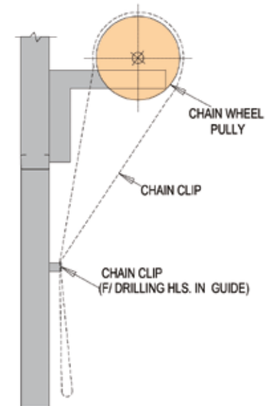
View X1 Showing Drive Chain
