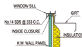
SECTION THRU' WINDOW SILL
