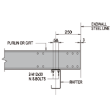
PURLIN/GIRT CONNECTION DETAIL At Lines 1 & 9
