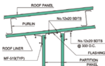
DETAIL 'G' TRANSVERSE SECTION SHOWING LONGITUDINAL PARTITION CONNECTION TO ROOF WITH LINER
