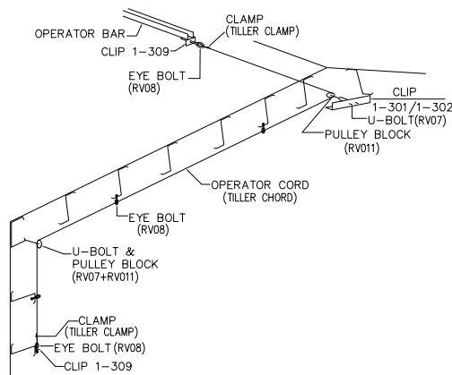
OPERATOR CORD ATTACHMENT SCHEMATIC
