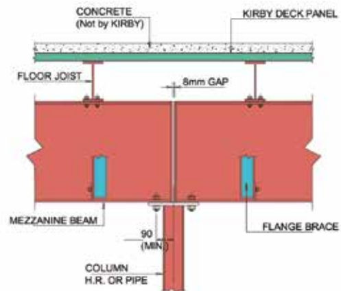
DETAIL - H MEZZANINE SUPPORT COLUMN
