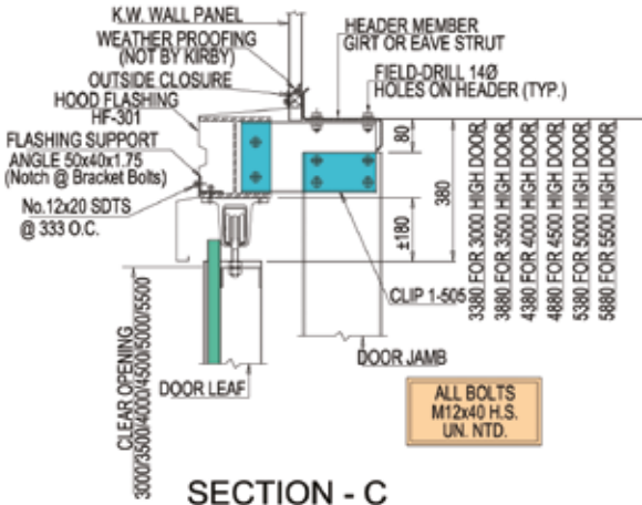
SECTION - C
