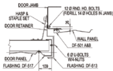
SECTION - M
