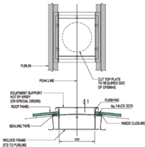
FRAMED OPENING AT PEAK DETAIL 'A'
