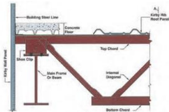
Open Web Steel Joist Connection Detail
