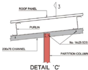
DETAIL 'C' TRANSVERSE SECTION SHOWING COLUMN & GIRT CONNECTION AT ROOF BETWEEN TWO FRAMES
