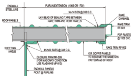
DETAIL 'D' PURLIN EXTENSION CANOPY WITH SOFFIT
