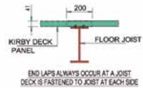
DETAIL - G DECK PANEL END LAPS
