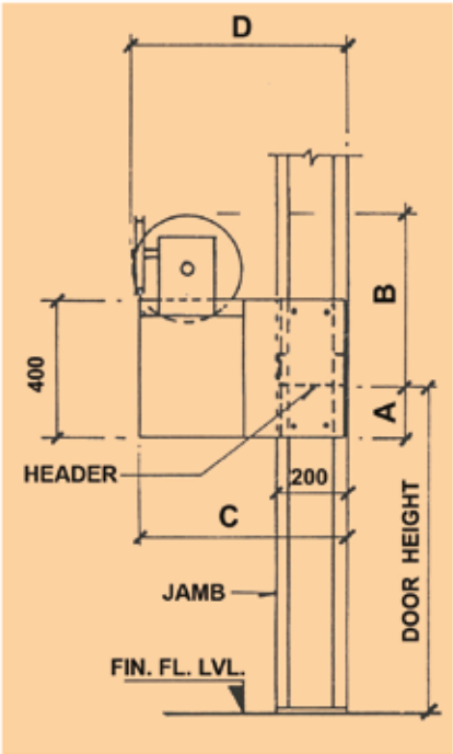
VIEW 'X-X'
