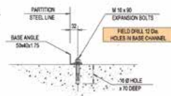
SECTION - 4
