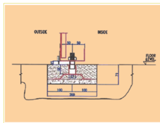
Detail of door leaf with bottom guide
