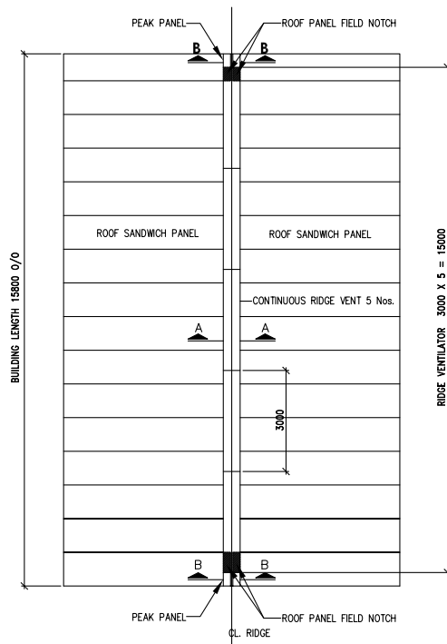
SAMPLE OF ROOF PLAN FOR RIDGE VENTILATOR (FOR INDICATION ONLY)
