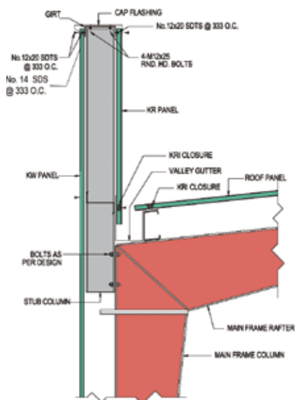
DETAIL 'A' SECTION AT SIDEWALL
