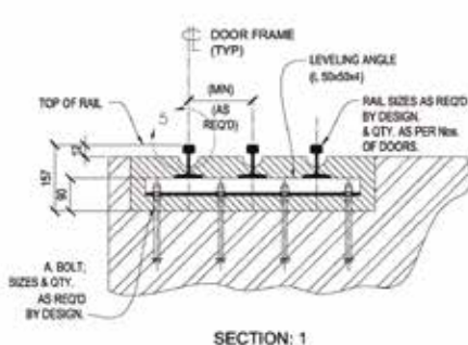
SECTION: 1
