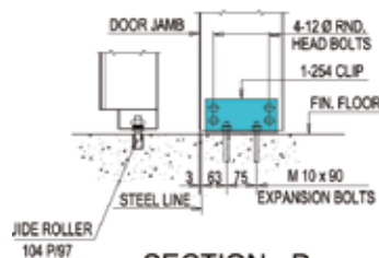
SECTION - P
