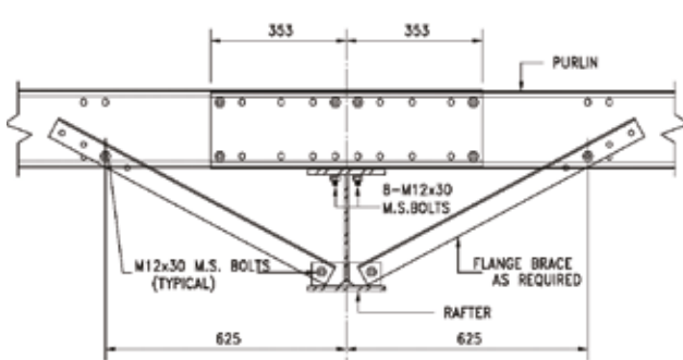
PURLIN CONNECTION DETAIL FROM GRID LINE 3-7
