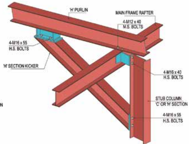
DETAIL 'B'
