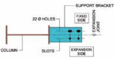
DETAIL OF SUPPORT BRACKET AT EXPANSION JOINT
