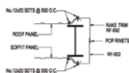
SECTION '3'
