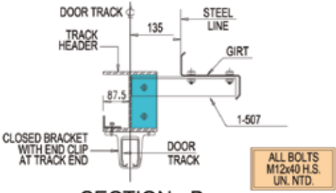
SECTION - B
