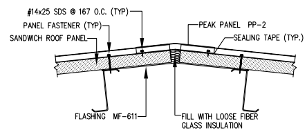
SECTION ON - B B (SECTION THRU PEAK PANEL)
