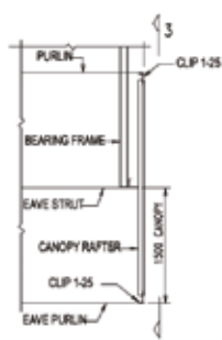
DETAIL 'C'
