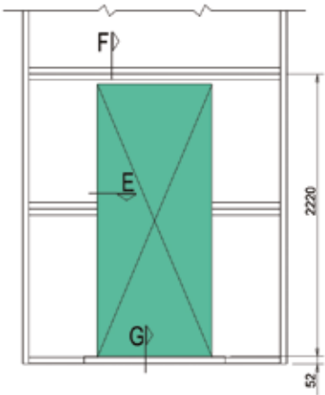
DOOR LEAF WITH 3070 WICKET DOOR
