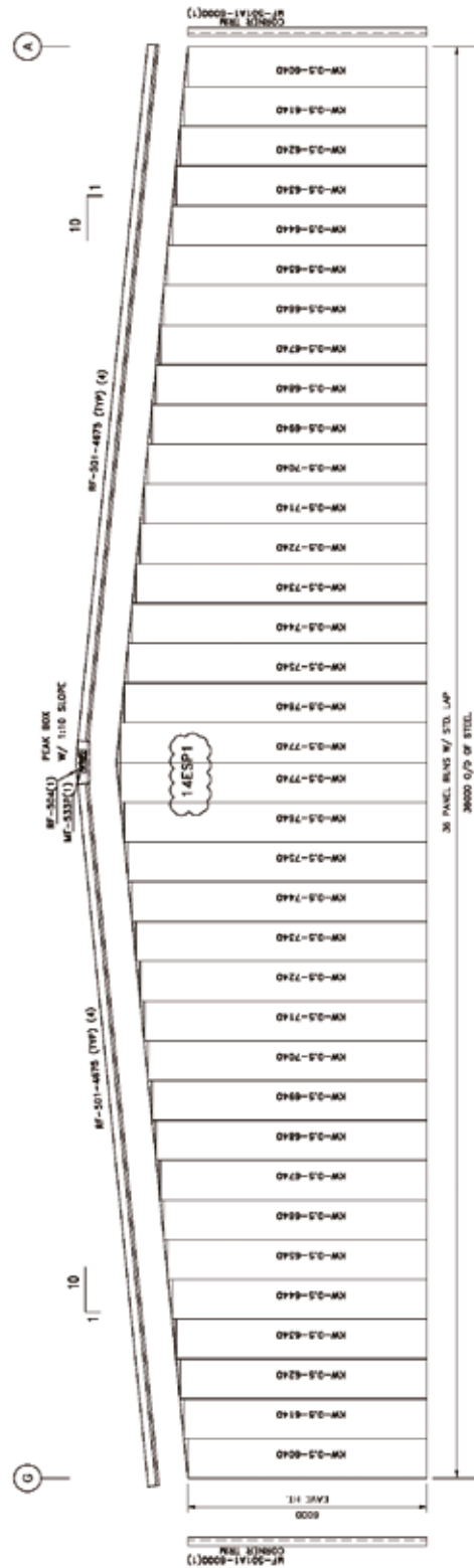
END WALL SHEET ELEVATION @ GL-1
