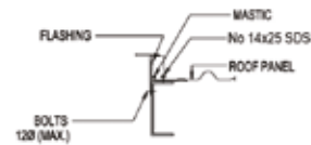
SECTION 3
