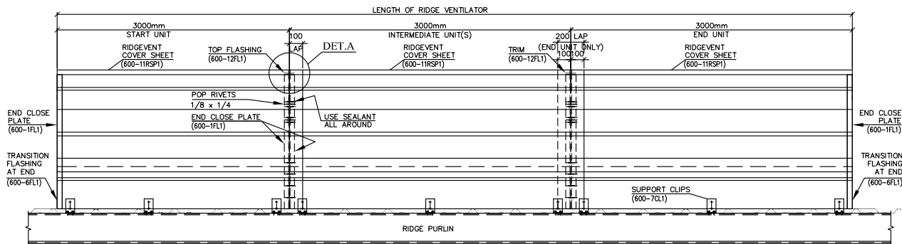
SIDE VIEW (CONTINUOUS RIDGE VENTILATORS)
