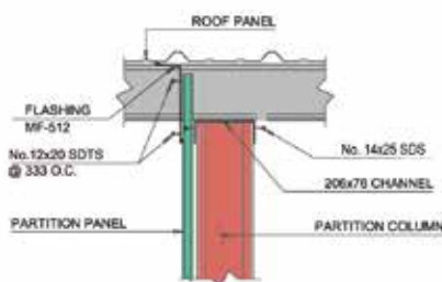
SECTION - 2
