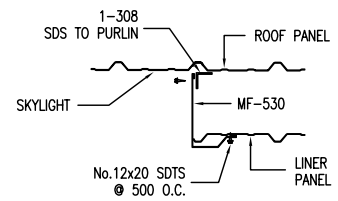
SECTION "2"
