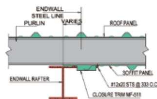
DETAIL 'H' OPEN ENDWALL FRAME WITH PURLIN EXTENSION CANOPY
