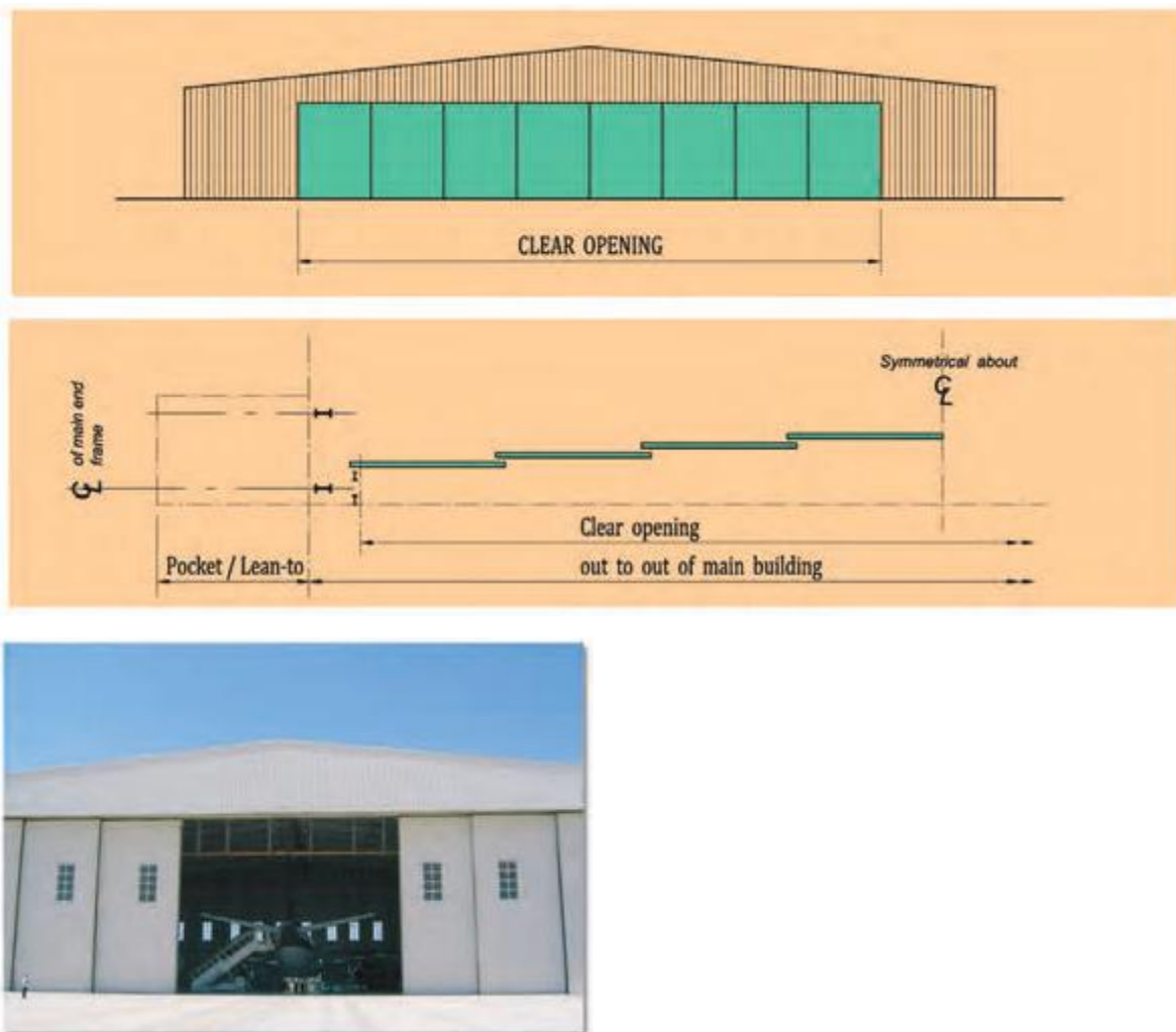
Aircraft hangar - Jordan
