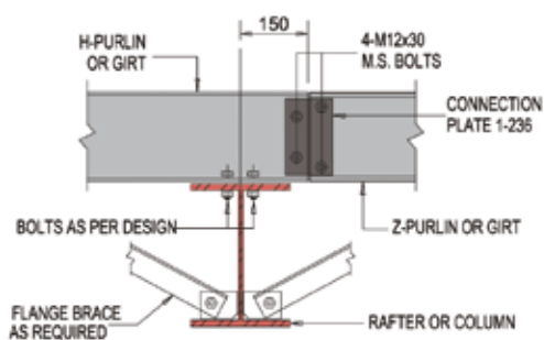
H & ZEE PURLIN/GIRT CONNECTION AT 107 & 165 LAPS
