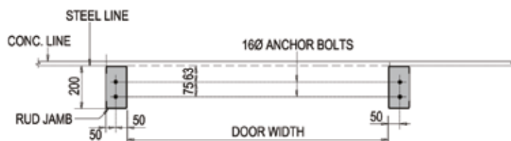
ANCHOR BOLT PLAN
