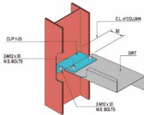
DETAIL 'A' FLUSH GIRT - 'H' SECTION COLUMN Flange Width = 150 mm
