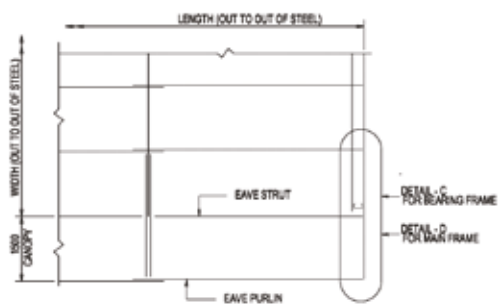
EAVE CANOPY
