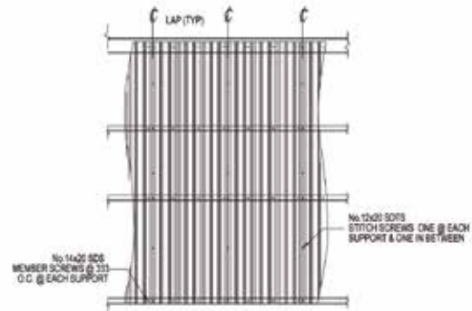
SCREW LAYOUT FOR LINER PANELS
