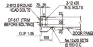
SECTION - G
