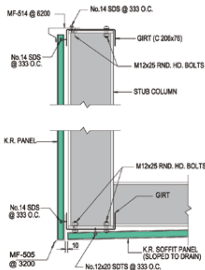
ENLARGED DETAILS
