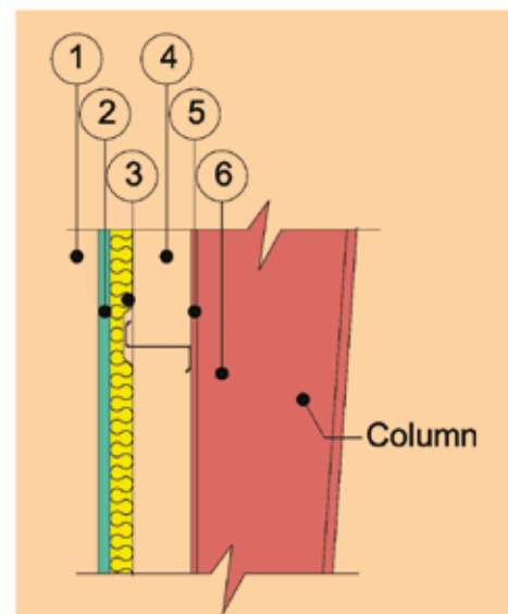
AT WALL
