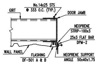
DOOR LEAF ERECTION (FOR 4500, 5000, 5500 & 6000 (AS NOTED) HIGH DOORS) RIGHT LEAF ERECTION - AS SHOWN LEFT LEAF ERECTION - OPP. HAND
