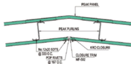
DETAIL 'F' SECTION THRU' PEAK
