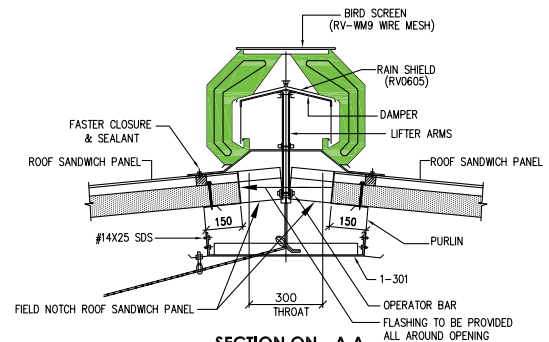
SECTION ON - A A (SECTION THRU RIDGE VENTILATOR)
