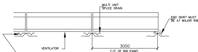
CONTINUOUS VENTILATOR INSTALLATION
