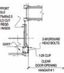
SECTION: R
