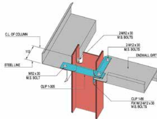
DETAIL 'H' BEARING FRAME - 'T' SECTION CORNER COLUMN
