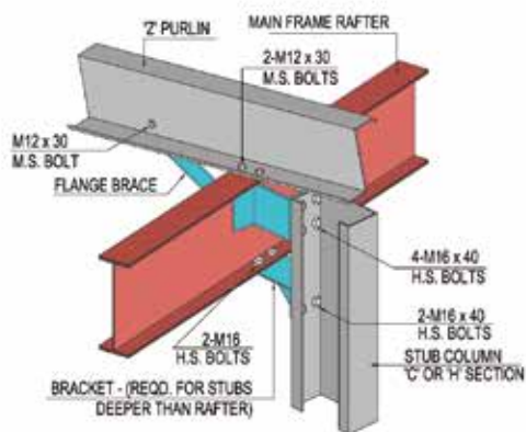
DETAIL 'C'
