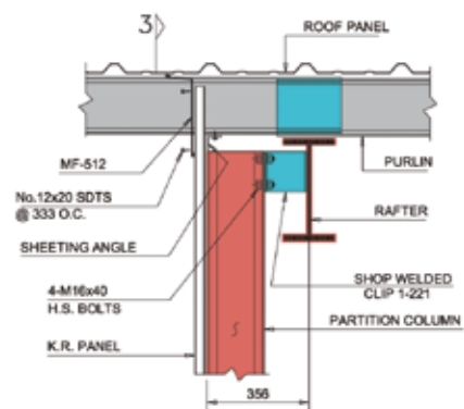
DETAIL 'D' LONGITUDINAL SECTION SHOWING PARTITION COLUMN CONNECTION TO RAFTER & FLASHING AT ROOF
