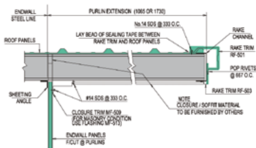
DETAIL 'E' PURLIN EXTENSION CANOPY WITHOUT SOFFIT
