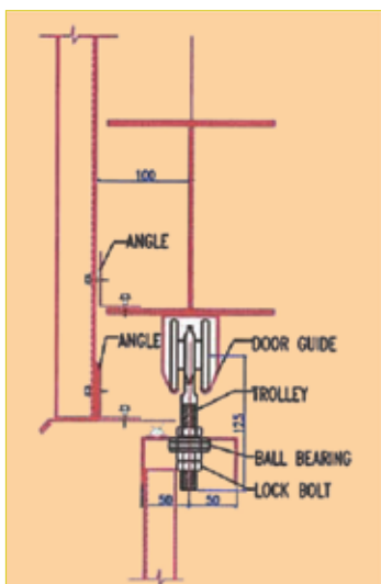
Detail of door leaf with top guide
