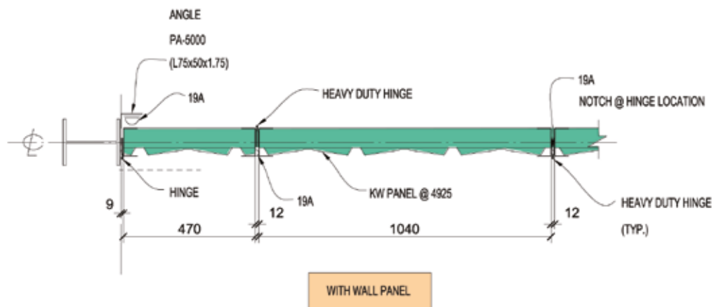
DETAIL - A1 FOLDING SLIDE DOOR LEAF
