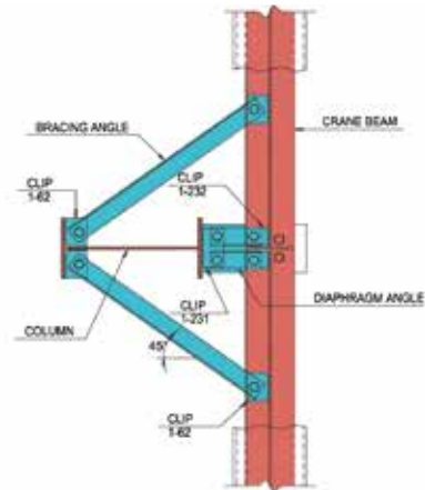
PLAN B-B
