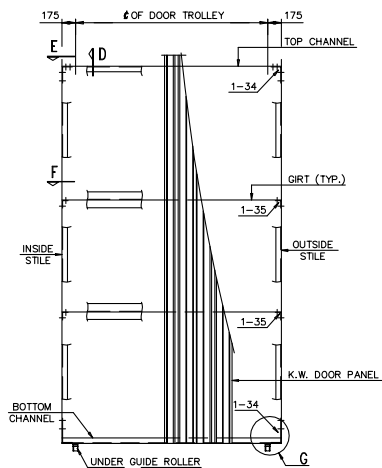
DOOR LEAF ERECTION (FOR 3000, 3500 & 4000 HIGH DOOR) RIGHT LEAF ERECTION - AS SHOWN LEFT LEAF ERECTION - OPP. HAND
