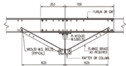
PURLIN CONNECTION DETAIL At Lines 2 & 8
