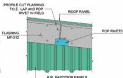
SECTION - 4
