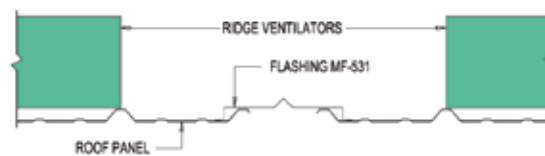
DETAIL 'E' AT RIDGE VENTILATOR
