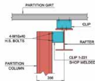
SECTION - 5
