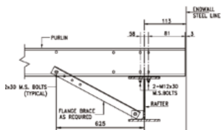
PURLIN CONNECTION DETAIL At Lines 1 & 7
