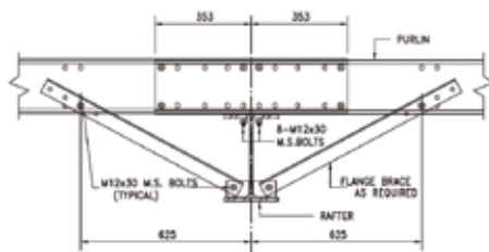
PURLIN CONNECTION DETAIL FROM GRID LINE 3 - 7
