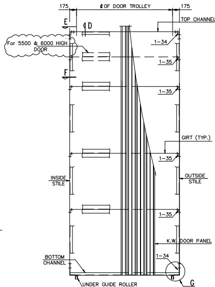
DOOR LEAF ERECTION (FOR 4500, 5000, 5500 & 6000 (AS NOTED) HIGH DOORS) RIGHT LEAF ERECTION - AS SHOWN LEFT LEAF ERECTION - OPP. HAND
