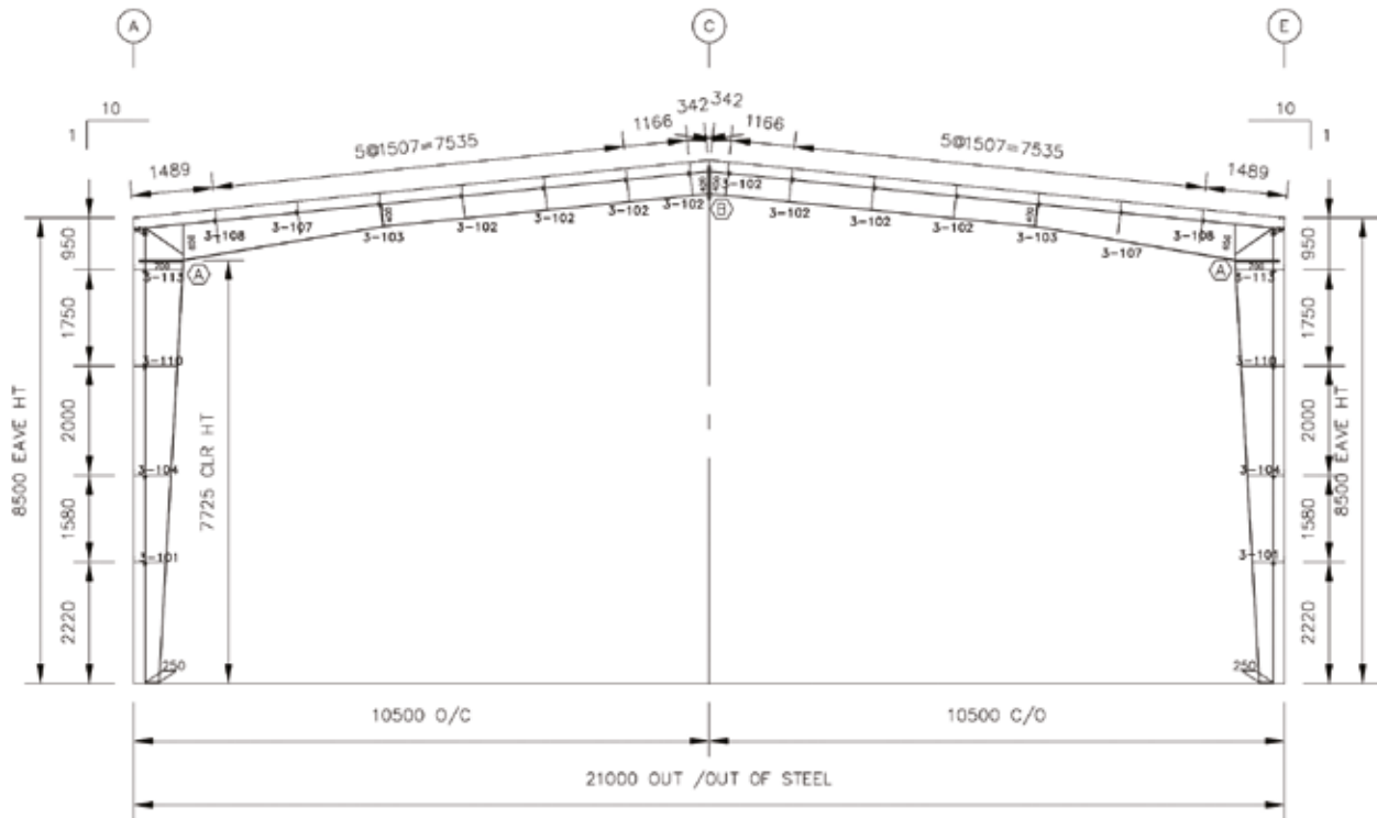
CROSS SECTION @ 2-6
