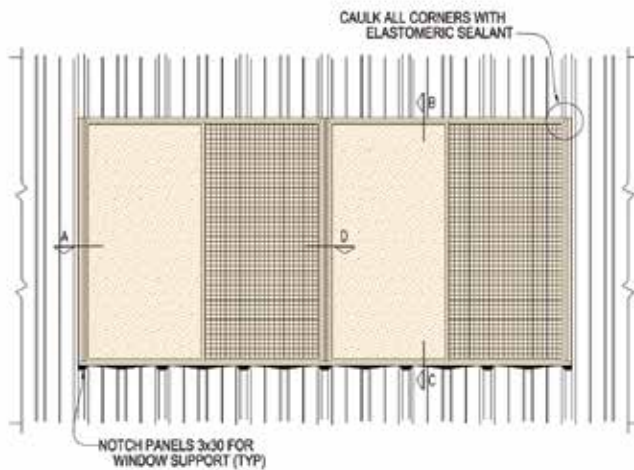
DOUBLE OR MULTIPLE WINDOW INSTALLATION
