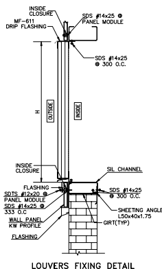
LOUVERS FIXING DETAIL BET. GIRTS W/ FRAMED OPENING FOR SINGLE SKIN WALL PANEL
