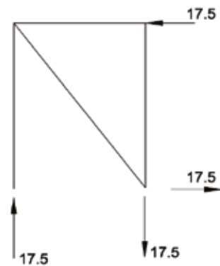
MAX BRACED BAY REACTIONS (KNS)
