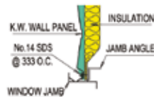
SECTION THRU' WINDOW JAMB
