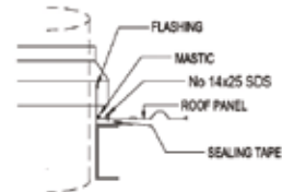
SECTION 2
