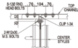
DETAIL - E
