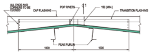
DETAIL 'E' AT PEAK
