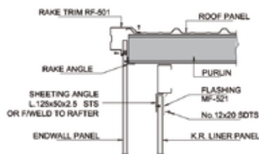
DETAIL 'D' SECTION AT BEARING FRAME ENDWALL RAFTER
