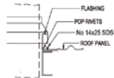
SECTION 4
