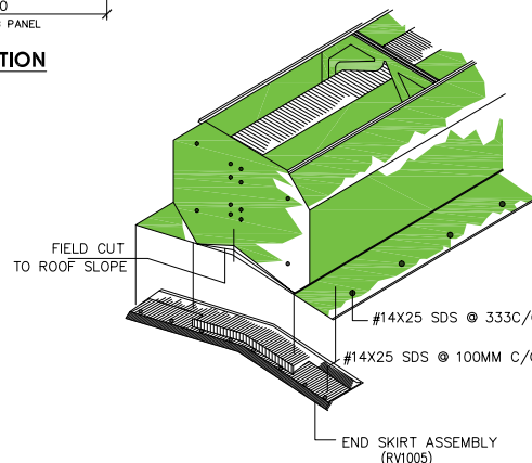
SINGLE AND/OR END UNIT INSTALLATION
