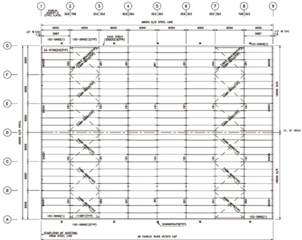
ROOF FRAMING ELEVATION
