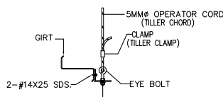
OPERATOR CORD ATTACHMENT TO GIRT
