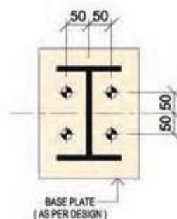
BOLT PLAN FOR INTERIOR MEZZANINE COLUMN
