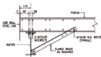
PURLIN CONNECTION DETAIL AT GRID LINE 1 & 9
