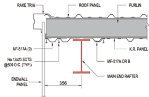
DETAIL L AT MAIN END WITHOUT WALL LINER
