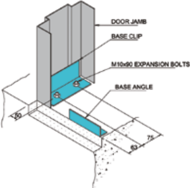
DETAIL AT 'Y'
