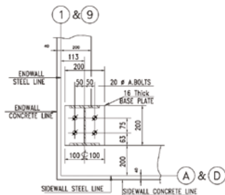
DETAIL 'B'
