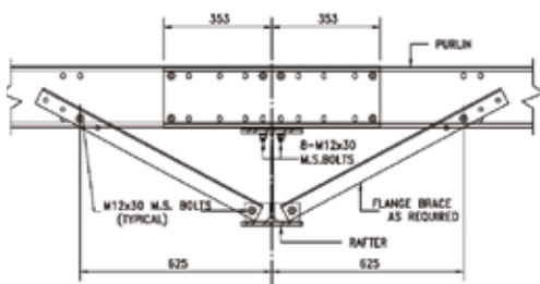
PURLIN CONNECTION DETAIL FROM GRID LINE 3 - 5
