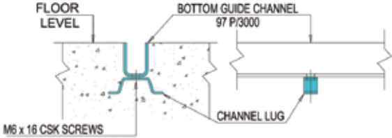
GUIDE CHANNEL ANCHORING DETAIL
