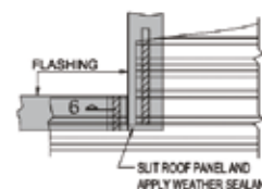
TYPICAL DETAIL AT CORNERS
