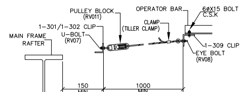
CORD ATTACHMENT DETAIL BET. OPERATOR BAR & 1-301 CLIP
