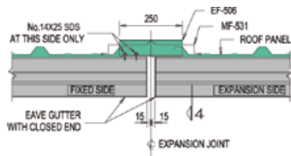
DETAIL 'D' AT EAVE GUTTER
