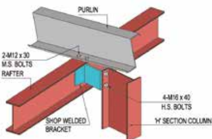
DETAIL 'B' RAFTER & PURLIN CONNECTION TO 1/2 SECTION INTERMEDIATE COLUMN
