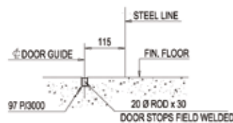
SECTION - Q
