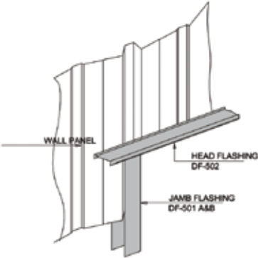
TRIM DETAIL AT 'X'
