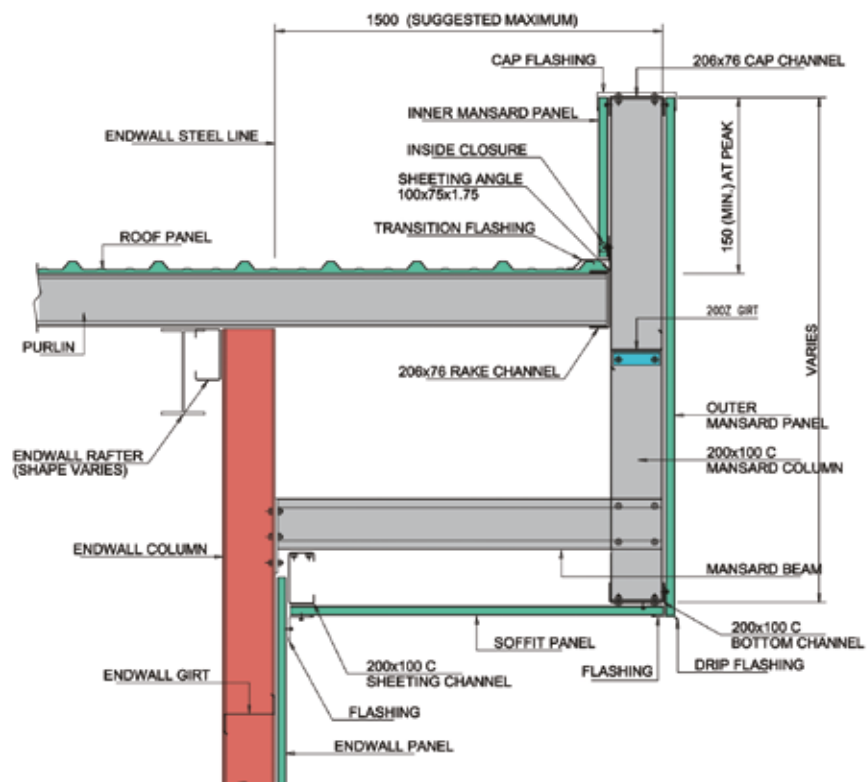
SECTION AT ENDWALL
