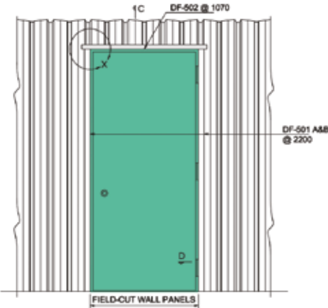
3'x7' WALK DOOR (914X2134)
