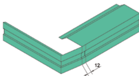
DETAIL 'E'
