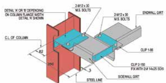
DETAIL 'K' MAIN FRAME ENDWALL CORNER DETAIL SIDEWALL GIRTS - FLUSH
