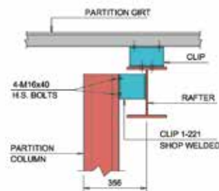
SECTION - 5
