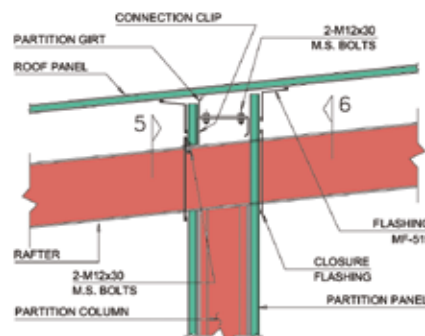
DETAIL 'F' TRANSVERSE SECTION SHOWING PARTITION SUPPORT & SHEETING BETWEEN EAVE AND PEAK
