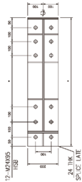
DETAIL "A"
