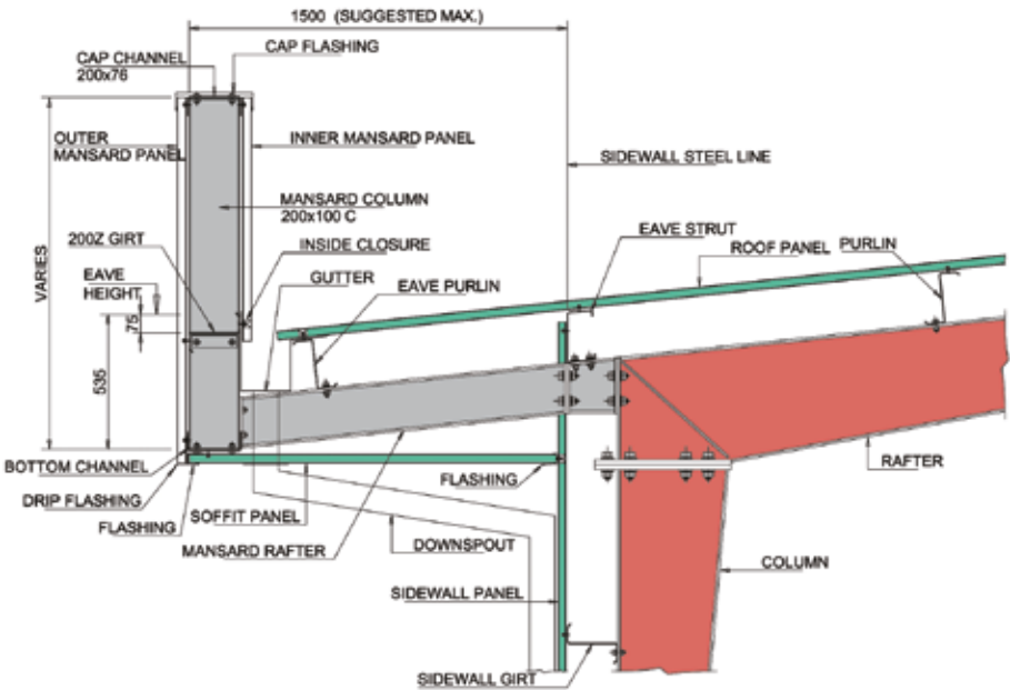
SECTION AT SIDEWALL
