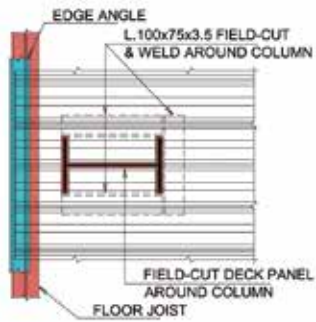
DETAIL - E PLAN AT RIGID FRAME COLUMNS
