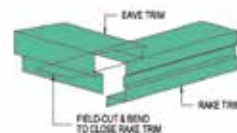
CORNER DETAIL
