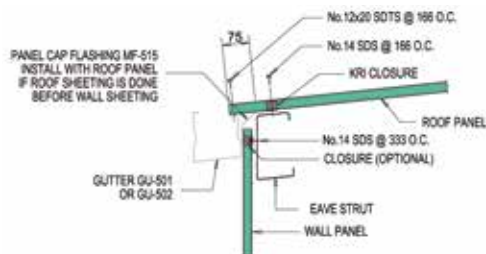
DETAIL 'A' SHEETED SIDEWALL
