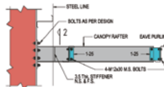
DETAIL 'C' AT RY-FRAME SIDEWALL OR ENDWALL
