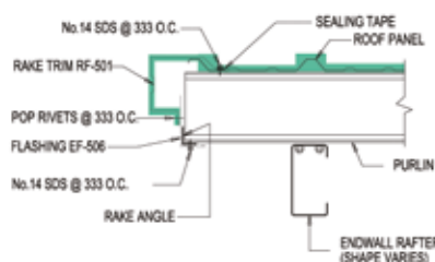
DETAIL 'D' OPEN ENDWALL
