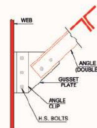
ANGLE BRACE CONNECTION
