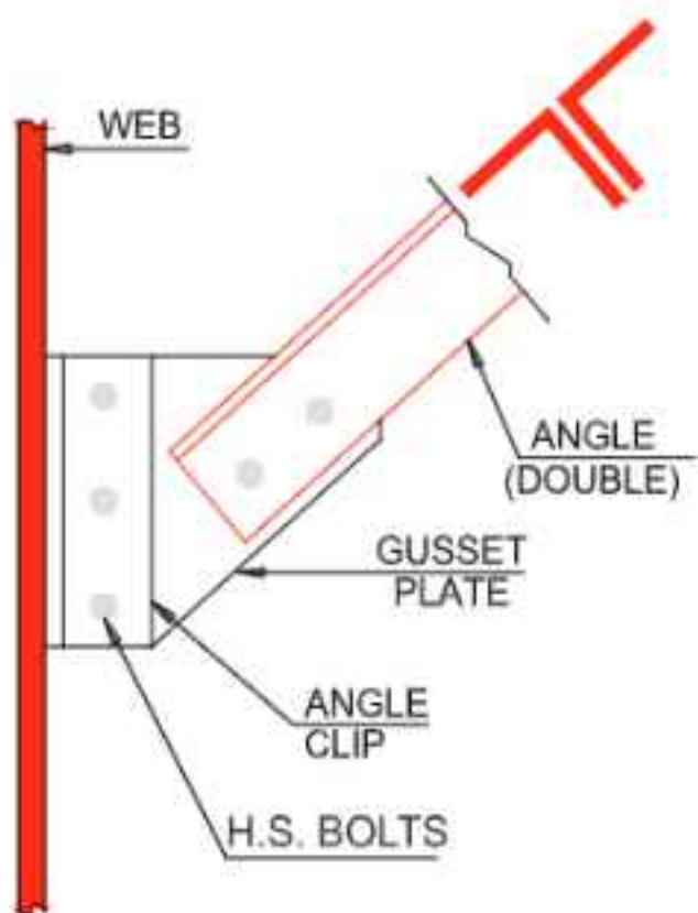
ANGLE BRACE CONNECTION
