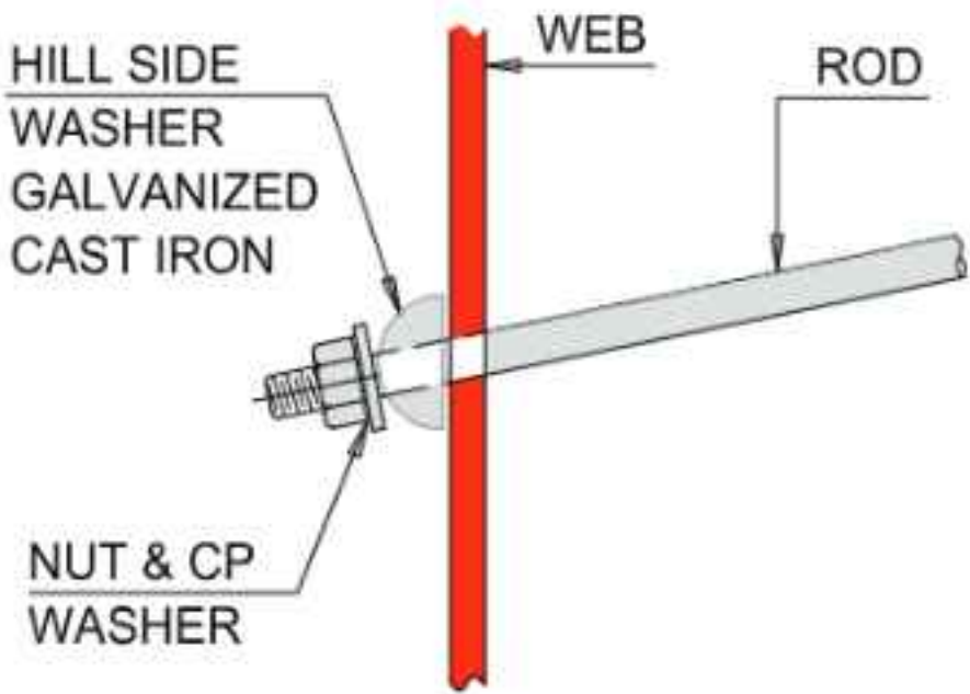
BRACE ROD CONNECTION
