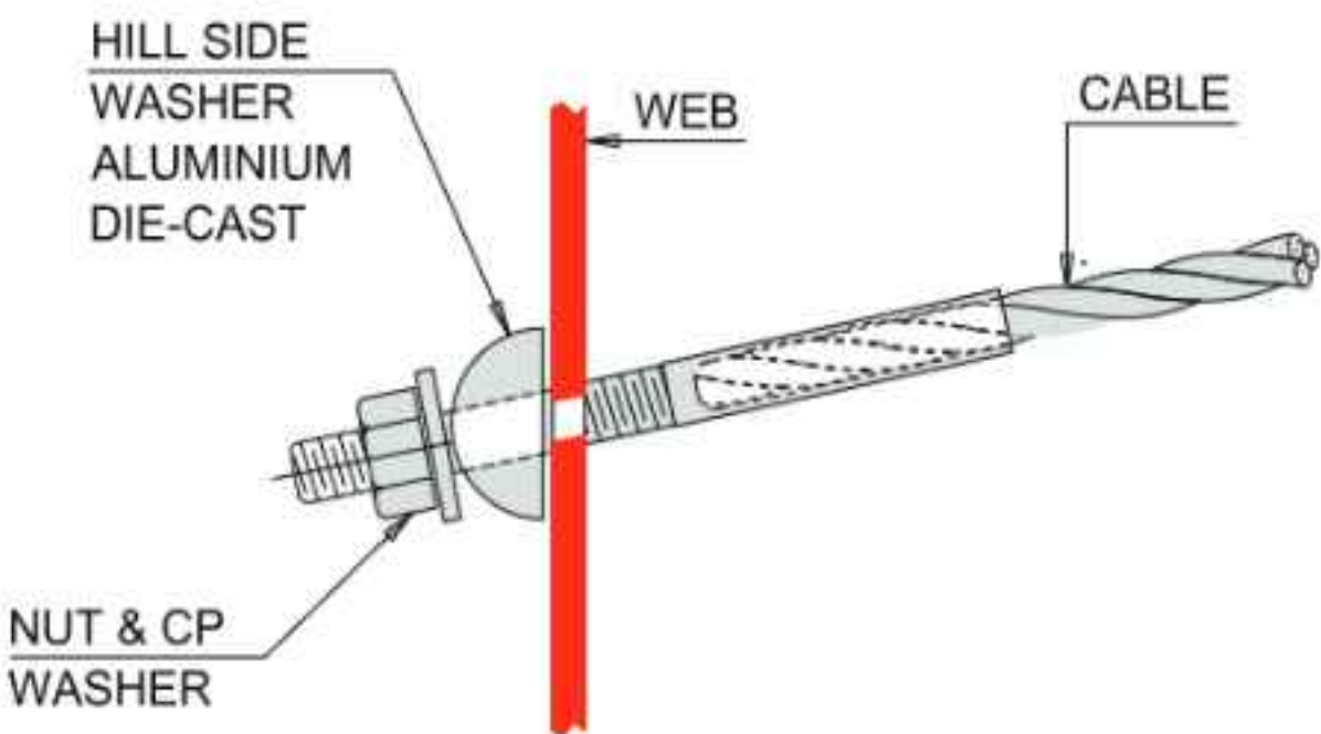
CABLE END CONNECTION
